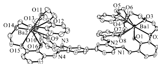
Figure 8. Molecular structure of 4\text{-Ba} . Perchlorate anions, solvent molecules, and hydrogen atoms have been omitted for clarity. Selected bond lengths [Å] and angles [°]: Ba1–O1 2.745(5), Ba1–O2 3.001(5), Ba1–O3 2.975(5), Ba1–O4 2.934(5), Ba1–O5 3.010(5), Ba1–O6 2.965(5), Ba1–O7 2.903(5), Ba1–O8 2.786(5), Ba2–O9 2.828(5), Ba2–O10 3.046(6), Ba2–O11 2.945(6), Ba2–O12 2.932(6), Ba2–O13 2.956(5), Ba2–O14 2.984(6), Ba2–O15 2.995(6), Ba2–O16 2.816(5); O1–Ba1–O6 156.66(15), O8–Ba1–O3 116.71(14), O7–Ba1–O3 171.01(15), O4–Ba1–O2 98.17(14), O6–Ba1–O2 147.28(14), O2–Ba1–O5 149.92(14), O16–Ba2–O11 122.12(17), O9–Ba2–O14 154.50(16), O12–Ba2–O15 119.58(17), O11–Ba2–O15 175.73(17), O13–Ba2–O10 152.92(16), O14–Ba2–O10 150.05(16).
