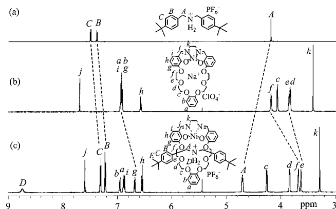
Figure 3. 1 H NMR spectra (600 MHz, CD 3 CN, 25 °C) of (a) 2-H ·PF 6 , (b) 1a ·Ni II ·Na(I), and (c) 3a-H ·PF 6 .
