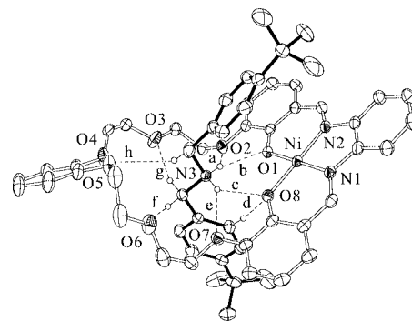
Figure 7. Molecular structure of 3\text{b}\cdot\text{H}\cdot\text{PF}_6 that indicates the intercomponent [\text{N}^+-\text{H}\cdots\text{O}] and [\text{C}-\text{H}\cdots\text{O}] hydrogen bonds. The nonhydrogen-bonding hydrogen atoms, disordered carbon atoms, and the counter anion have been omitted for clarity. Hydrogen bonding geometries: [\text{X}\cdots\text{O}] , [\text{H}\cdots\text{O}] distances [Å] and [\text{X}-\text{H}\cdots\text{O}] angles [°] are (a) 2.906, 2.148, 141.5; (b) 2.829, 2.074, 140.7; (c) 2.858, 2.127, 137.8; (d) 3.498, 2.572, 162.1; (e) 2.920, 2.141, 144.4; (f) 3.408, 2.545, 149.7; (g) 3.259, 2.329, 162.8; (h) 3.323, 2.575, 134.9.
