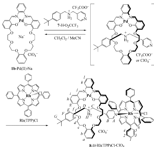
Scheme 3. Synthesis of tetraphenylporphyrin-stoppered [2]rotaxane 8 ·H·Rh(TPP)Cl·ClO 4 .
