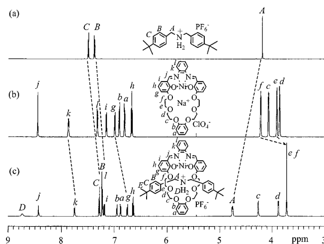
Figure 4. 1 H NMR spectra (600 MHz, CD 3 CN, 25 °C) of (a) 2-H ·PF 6 , (b) 1b ·Ni II ·Na(I), and (c) 3b-H ·PF 6 .
