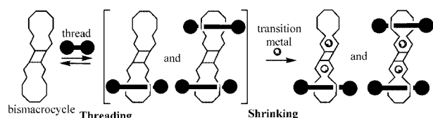
Figure 2. Graphical representation of the [2]rotaxane and bis[2]rotaxane when using the bismacrocycle and the “threading-followed-by-shrinking” approach.
