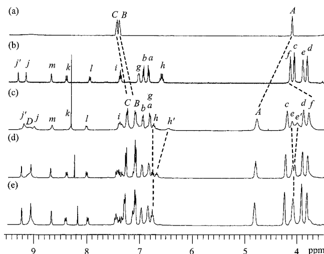
Figure 5. ^1\text{H} NMR spectra (400 MHz, [\text{D}_6]\text{DMSO} ) of (a) 2\text{-H}\cdot\text{PF}_6 , (b) 4\text{-Pd}^{\text{II}}\cdot\text{Na}(\text{I}) , and 6\text{-2H}\cdot 2\text{ClO}_4 recorded at temperatures of (c) 298 K, (d) 323 K, and (e) 353 K.
