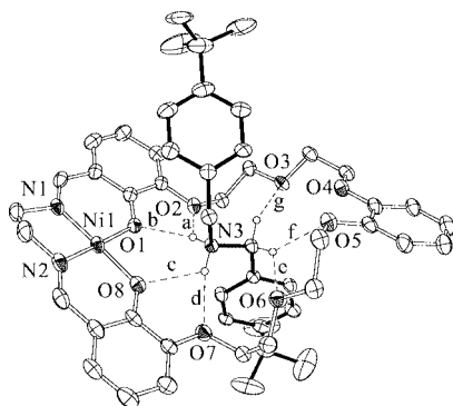
Figure 6. One molecular structure of 3\text{a}\cdot\text{H}\cdot\text{PF}_6 that indicates the intercomponent [\text{N}^+-\text{H}\cdots\text{O}] and [\text{C}-\text{H}\cdots\text{O}] hydrogen bonds. The other rotaxane molecule, the nonhydrogen-bonding hydrogen atoms, disordered carbon atoms, and the counter anion have been omitted for clarity. Hydrogen bonding geometries: [\text{X}\cdots\text{O}] , [\text{H}\cdots\text{O}] distances [Å] and [\text{X}-\text{H}\cdots\text{O}] angles [°] are (a) 3.067, 2.348, 136.8; (b) 2.840, 2.032, 148.6; (c) 2.737, 2.207, 117.1; (d) 2.892, 2.008, 166.8; (e) 3.264, 2.523, 134.0; (f) 3.429, 2.580, 147.6; (g) 3.185, 2.318, 149.9.
